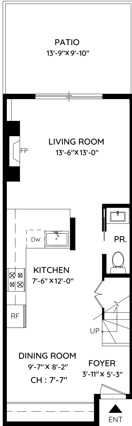
MAIN FLOOR 510 SQ.FT. CH: 10'-0"
